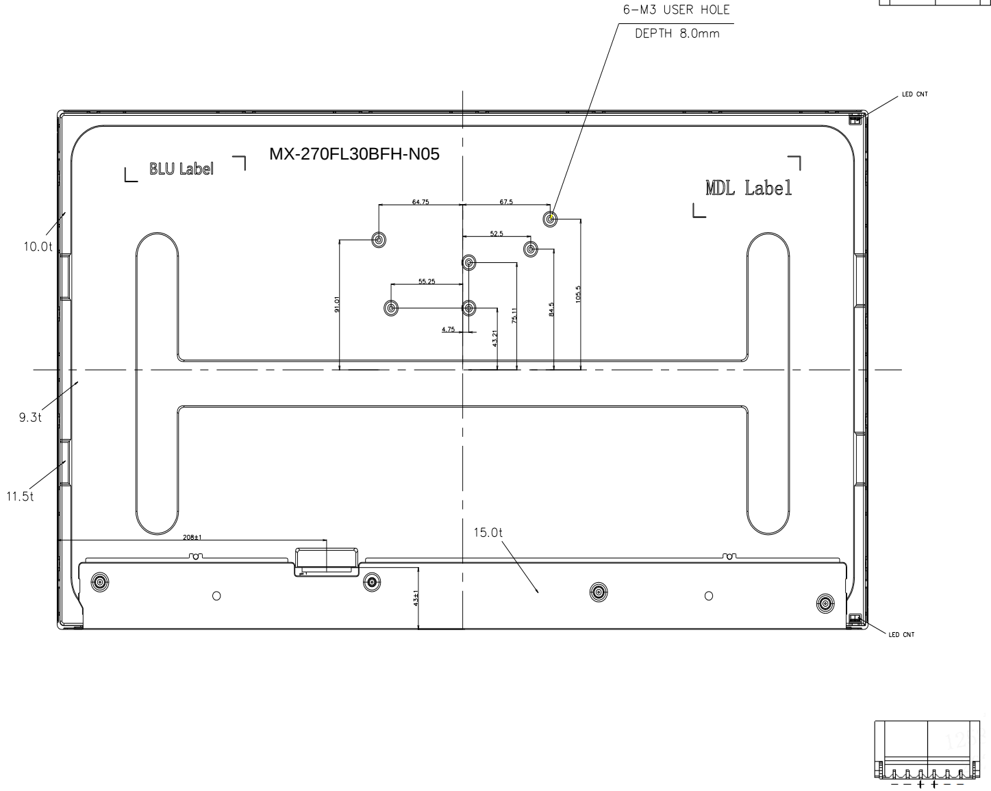
Figure 6. TFT-LCD Module Outline Dimensions (Rear view)
