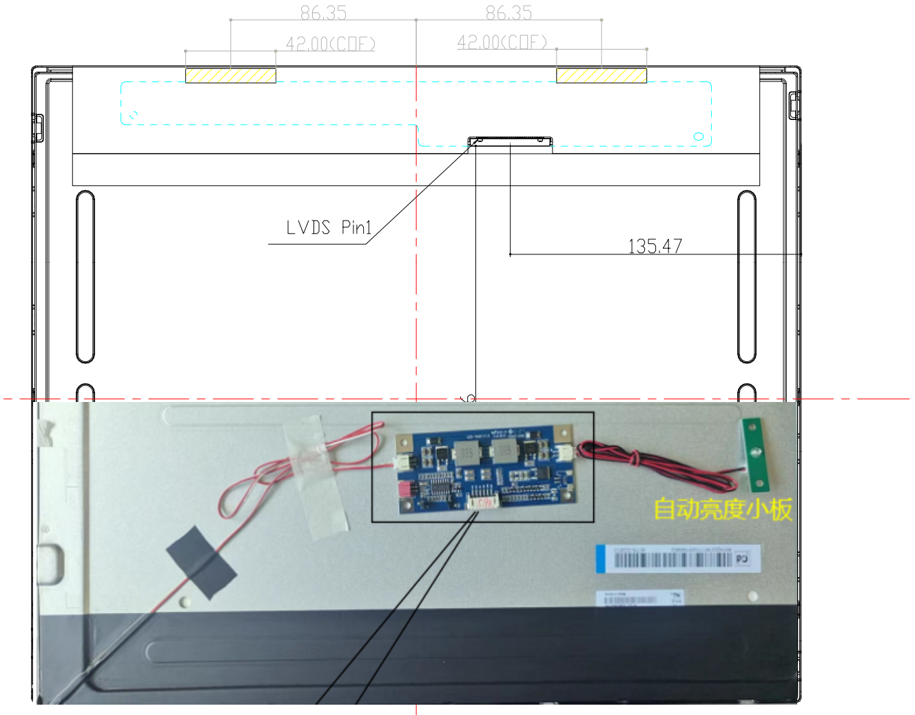
< Figure 2. TFT-LCD Module Outline Dimensions (Rear View) >
