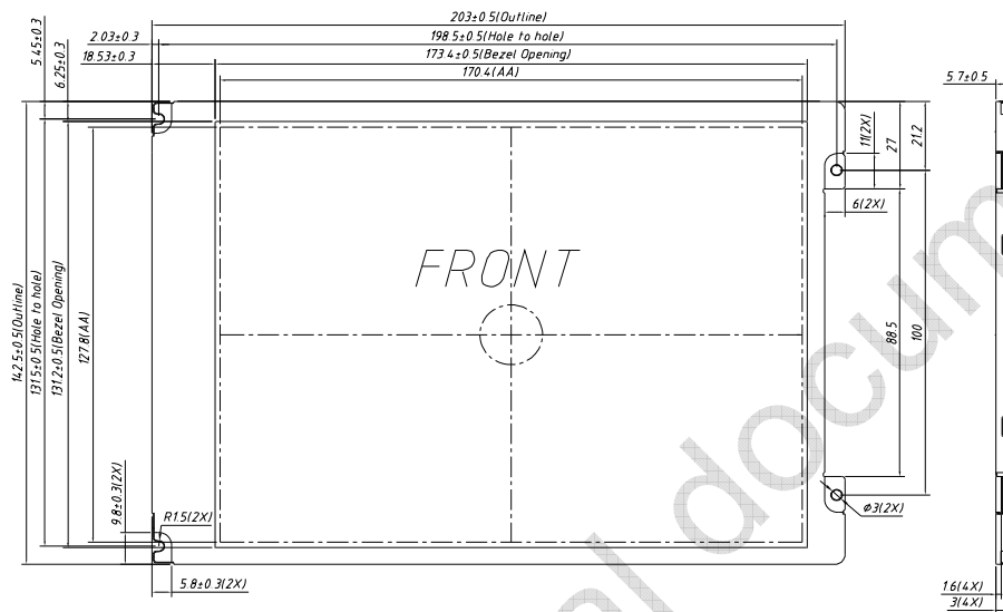
Figure 15 Outline Drawing (Front Side)
