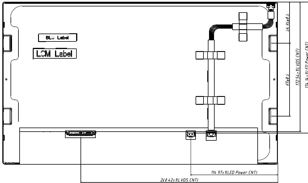
Figure 1 Reference Outline Drawing (Back Side)
