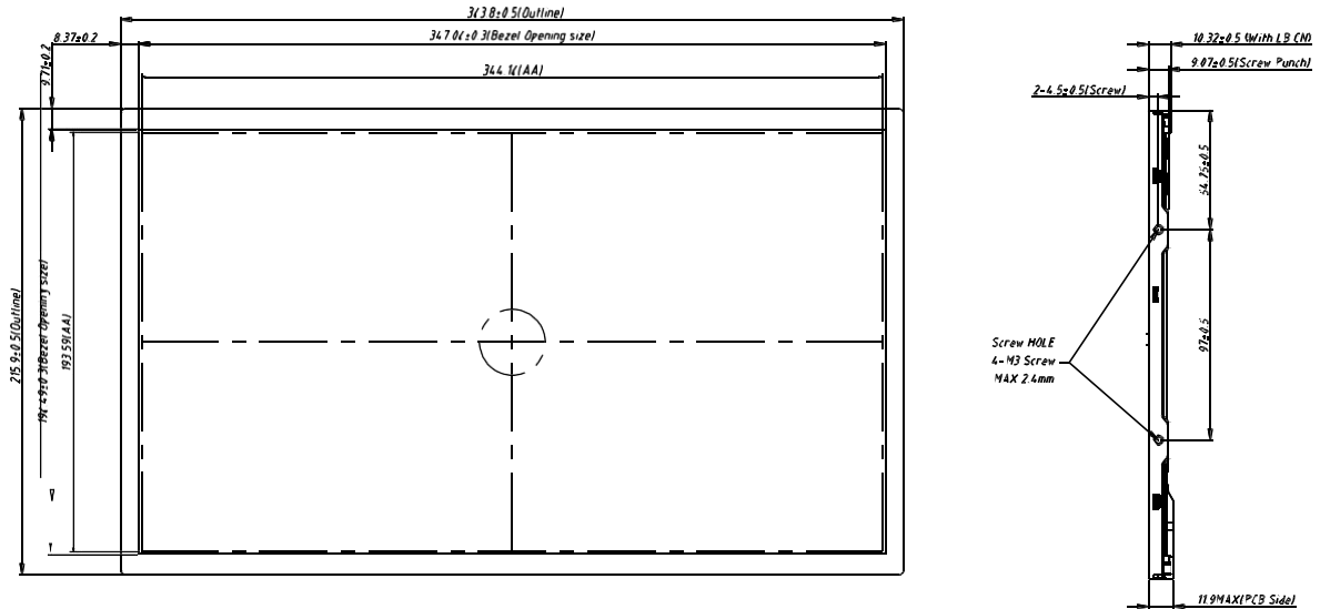
Figure 1 Reference Outline Drawing (Front Side)
