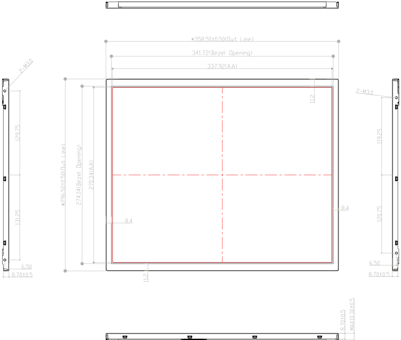
< Figure 1. TFT-LCD Module Outline Dimensions (Front View) >
