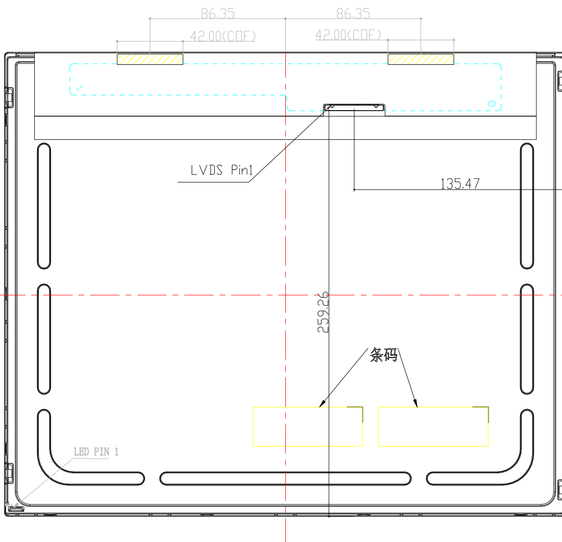
< Figure 2. TFT-LCD Module Outline Dimensions (Rear View) >
