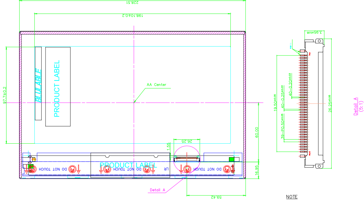
Figure 2. TFT-LCD Module Outline Dimensions (Rear view)
