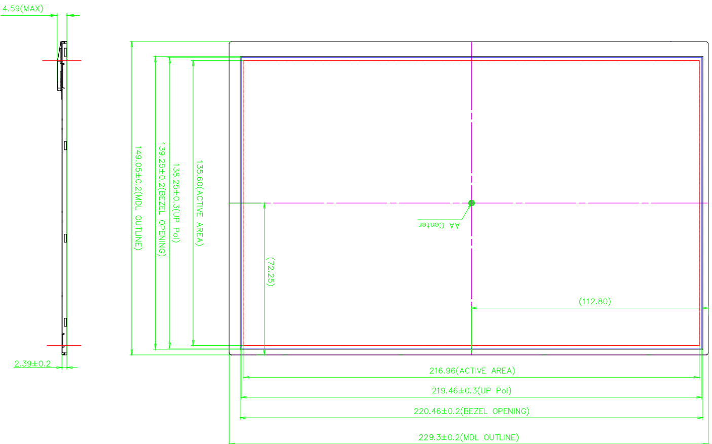
Figure 1. TFT-LCD Module Outline Dimension (Front View)
