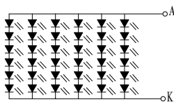
Backlight 6串6并 36LED Circuit
