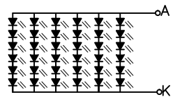
Backlight 6串6并 36LED Circuit
