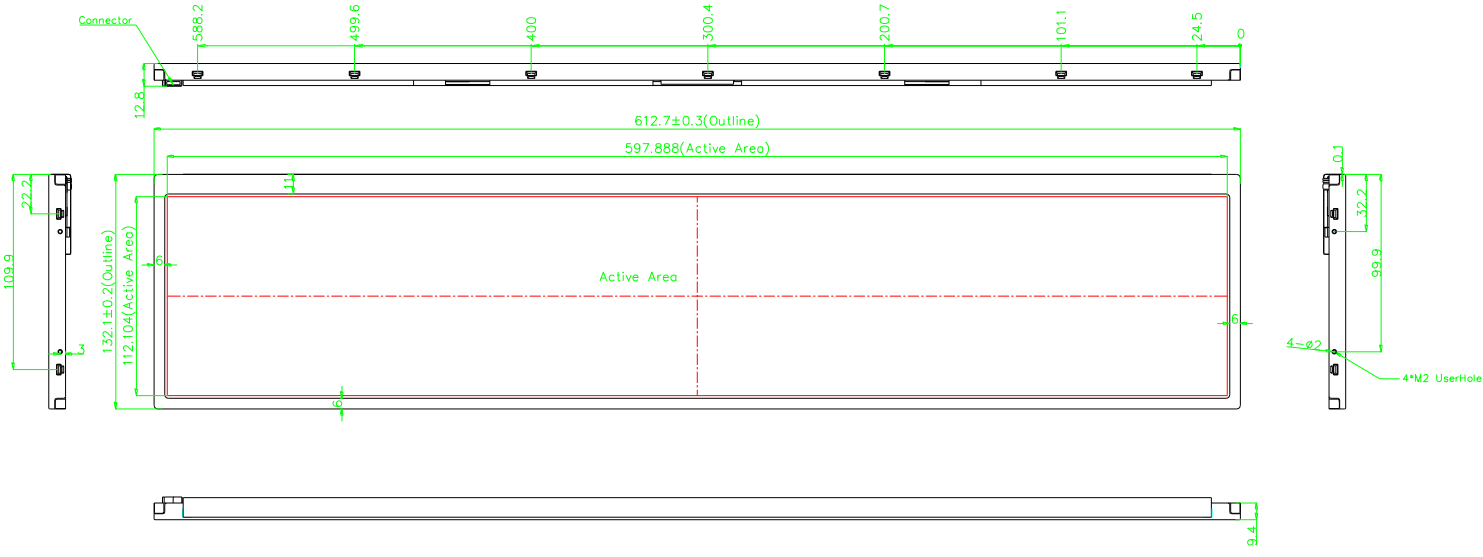
Figure 1. TFT-LCD Module Outline Dimensions (Front view)
