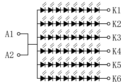
Backlight LED Circuit 8串6并 48LED VF:22.4-25.6V IF:120MA
